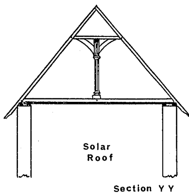
FIG. 3 Section of the old Hall and the Solar Roof.
